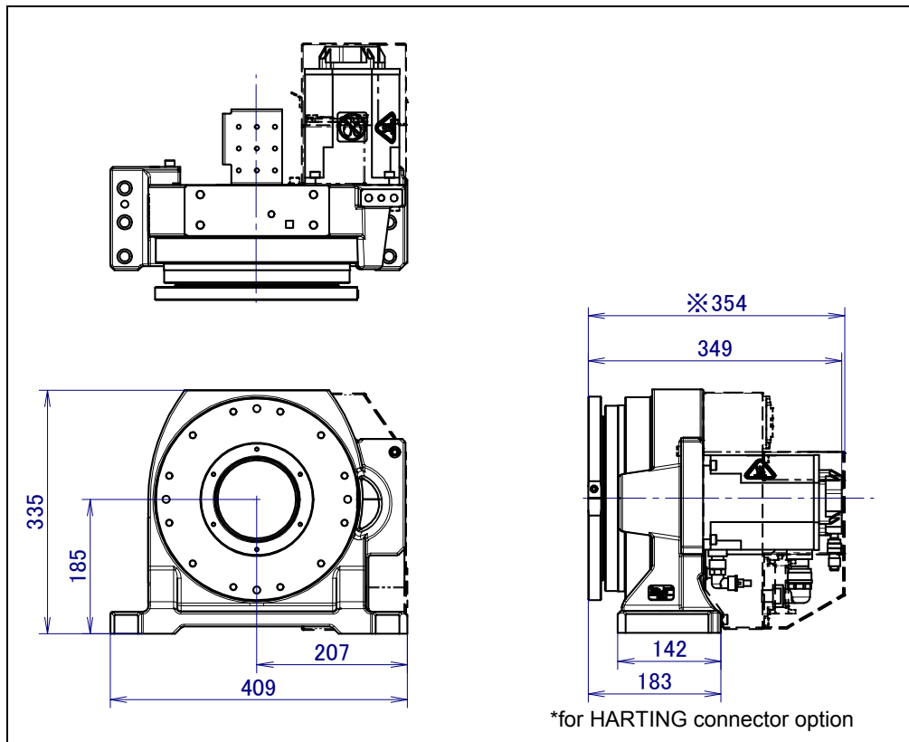
Fig. 3.2 (a) External dimensions of the 1-axis positioner
