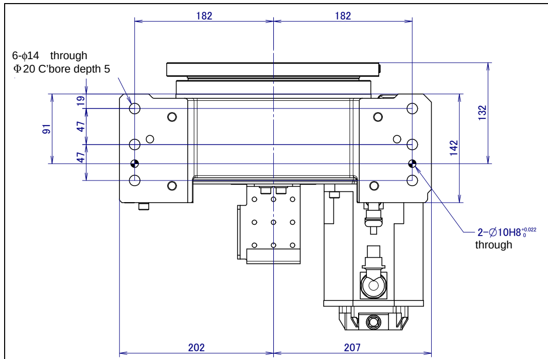
Fig. 1.2 (a) Dimensions of the positioner base
