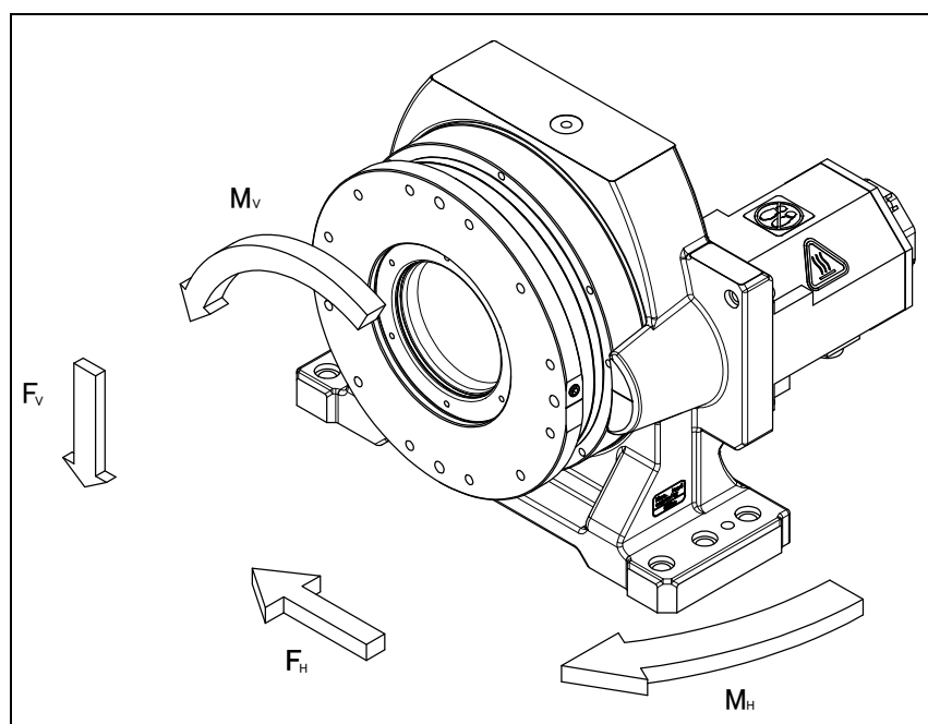
Fig. 1.2.1 (c) Force and moment that acts on J1 base
