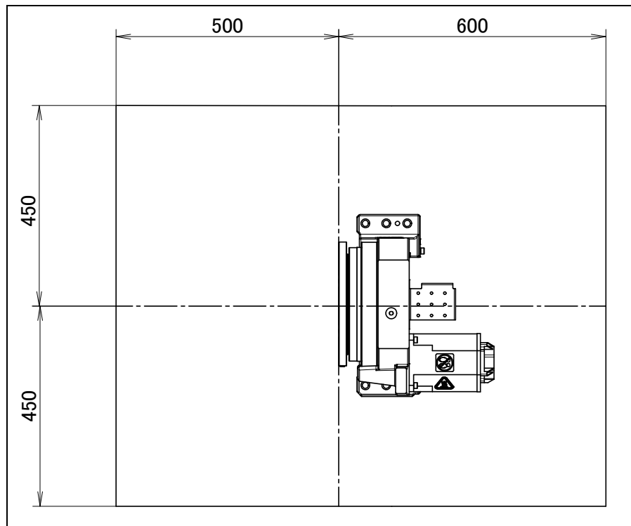
Fig. 1.3 (a) Maintenance area
