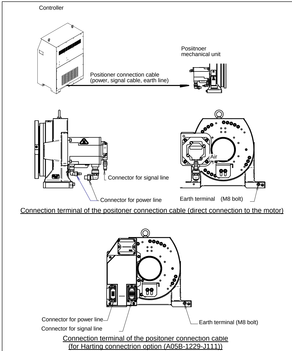
fig. 2.1 (a) Cable connection
