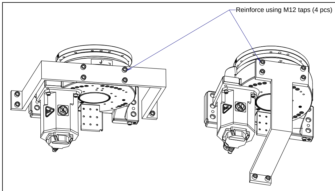
Fig. 1.2.1 (b) Reinforcement for the wall mount
