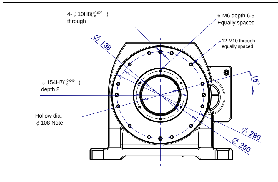
Fig. 4.1 (a) Equipment mounting faces of 1-axis positioner
