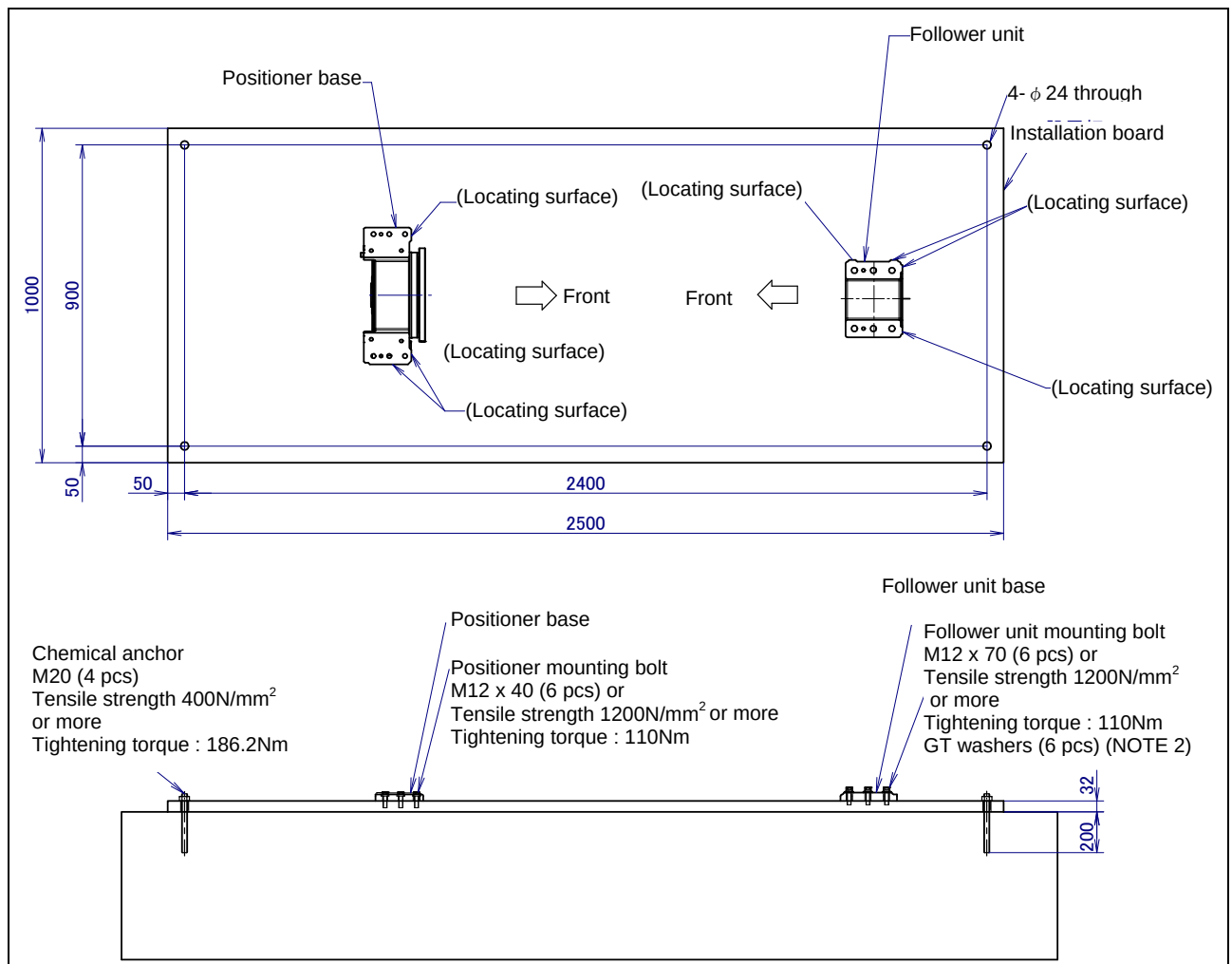
Fig. 1.2.1 (a) Example of installing the positioner
