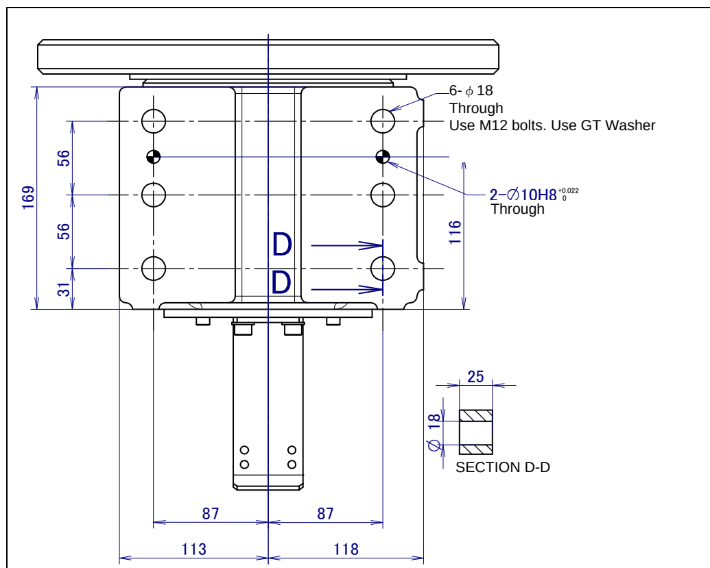
Fig. 1.2 (b) Dimensions of the base of the positioner follower unit (insulated flange)
