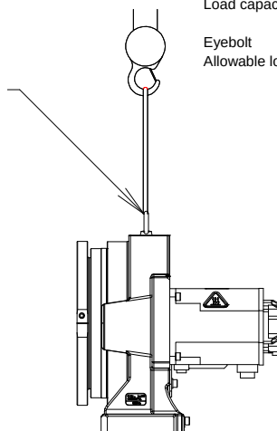
Fig. 1.1 (a) Transportation using a crane
