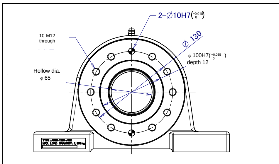
Fig. 4.1 (c) External dimensions of follower unit (non-insulated flange) (option)
