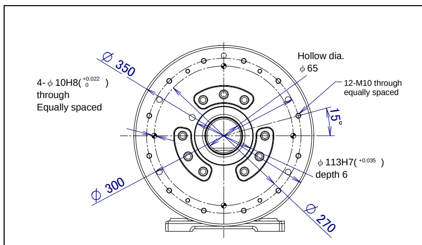
Fig. 4.1 (b) External dimensions of follower unit (insulated flange) (option)
