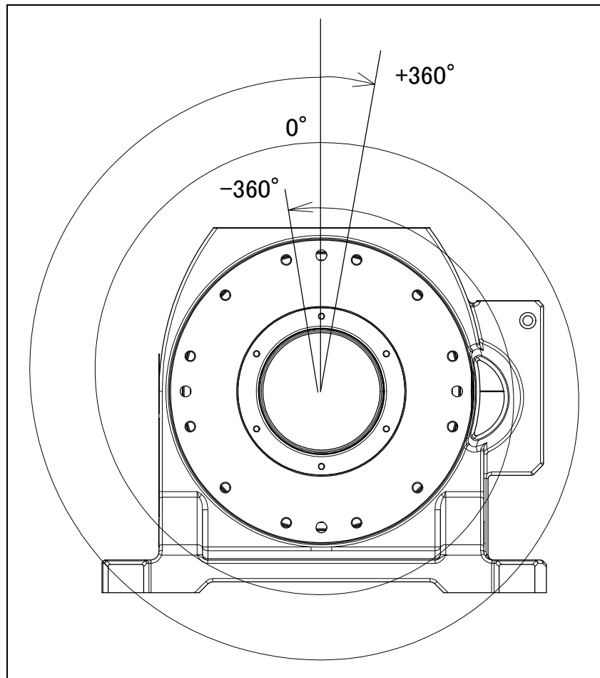
Fig. 3.3 (a) J1-axis motion limit
