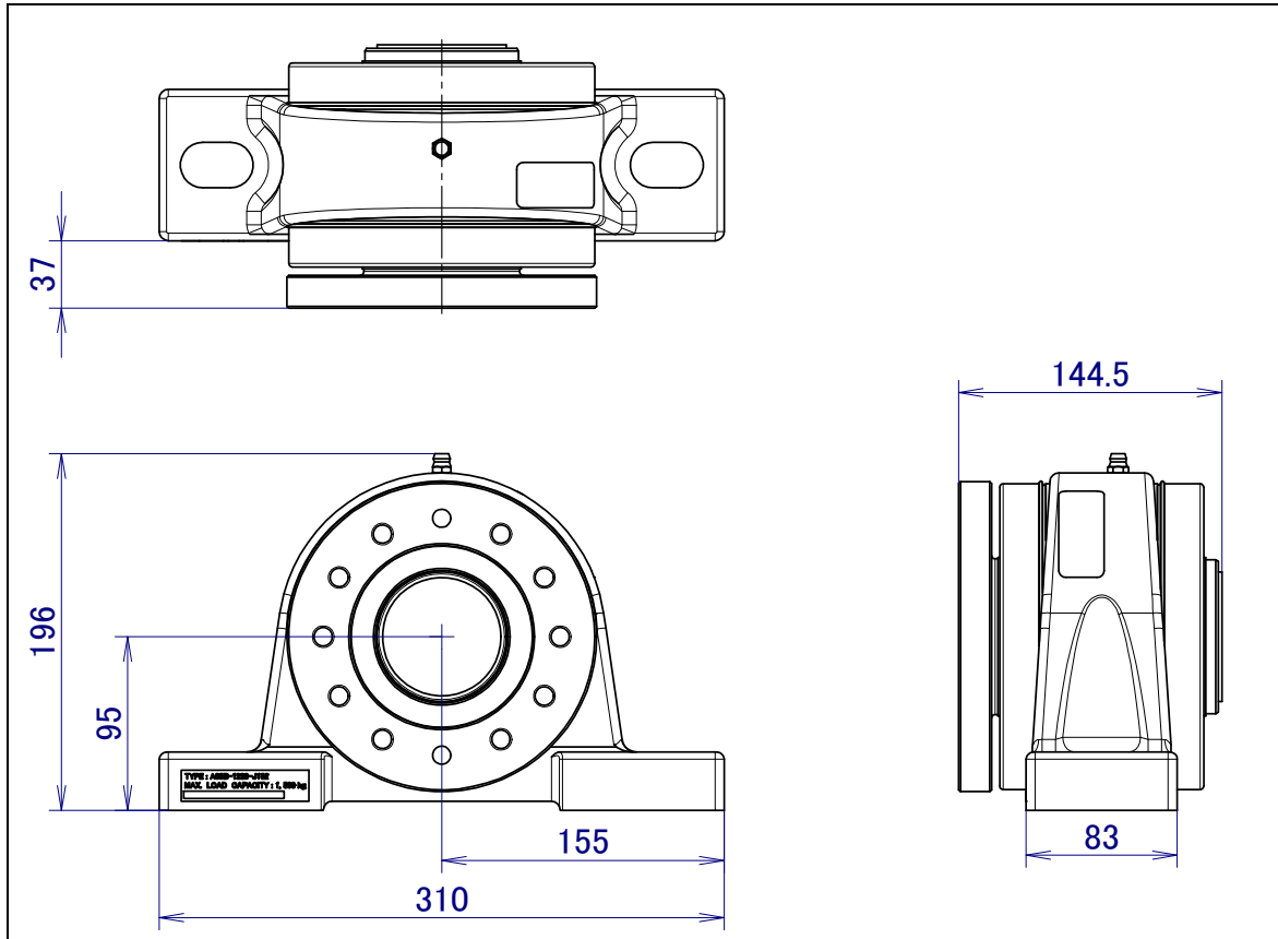
Fig. 3.2 (c) External dimension of the follower unit (without insulated flange) (option)
