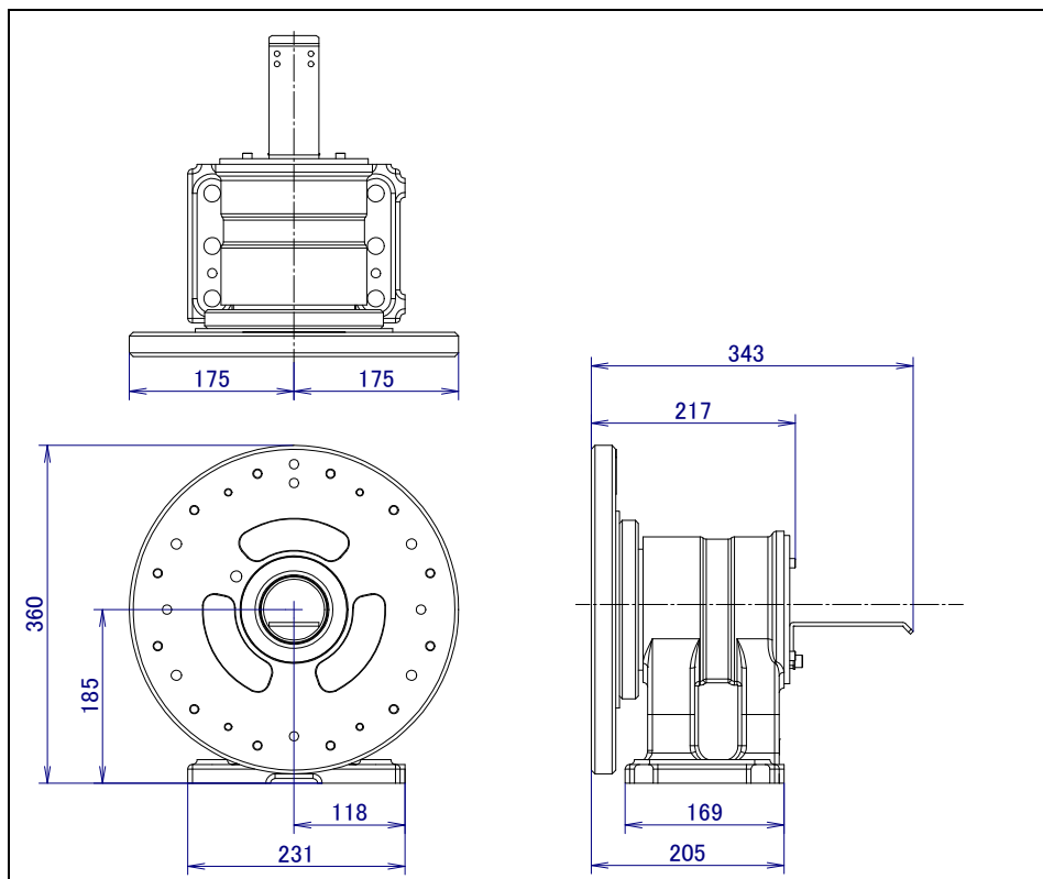
Fig. 3.2 (b) External dimension of the follower unit (with insulated flange) (option)
